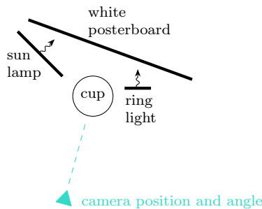
Figure 3: Birds eye view diagram of light setup including approximate location of camera lens during shooting. Diagram is not necessarily to scale.
