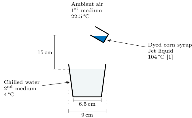
Figure 2: Diagram of the setup used for the picture. All values in this diagram are approximate [1].
